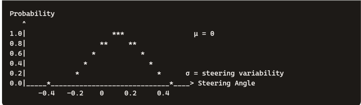
Fig. 5. Gaussian steering-angle probability density function used in AUROUAV. The diagram illustrates the normalized steering-angle distribution modeled as a univariate Gaussian with mean \mu = 0 and standard deviation \sigma , representing steering variability. The bell-shaped curve captures the likelihood of selecting a particular steering angle during navigation, with the highest probability concentrated at zero, corresponding to straight-line motion. Probability decreases symmetrically as the steering angle deviates from the mean, enforcing smooth, human-like control while allowing controlled variability for maneuvering. This probabilistic formulation forms the basis of the stochastic steering policy used in MPC and reinforcement-learning-based adaptation.
