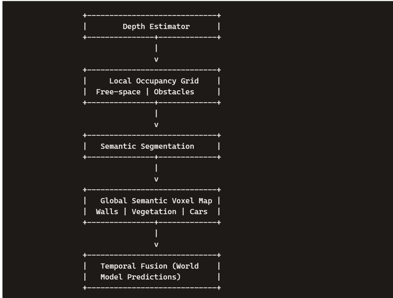
Fig. 9. Deep mapping architecture integrating geometric, semantic, and temporal scene understanding in AUROUAV. The diagram illustrates the hierarchical mapping pipeline that transforms raw depth and semantic information into rich spatial representations for navigation. Depth estimation produces geometric structure that is converted into a local occupancy grid encoding free-space and obstacles. Semantic segmentation provides pixel-wise class labels that are fused into a global semantic voxel map, enabling the system to distinguish between structural elements such as walls, vegetation, and vehicles. Temporal fusion incorporates predictions from the world-model subsystem, combining free-space forecasts and obstacle-motion dynamics with the geometric and semantic maps. This multi-layered mapping framework yields a unified, temporally consistent representation of the environment, supporting robust planning and safety-aware decision-making in GNSS-denied conditions.
