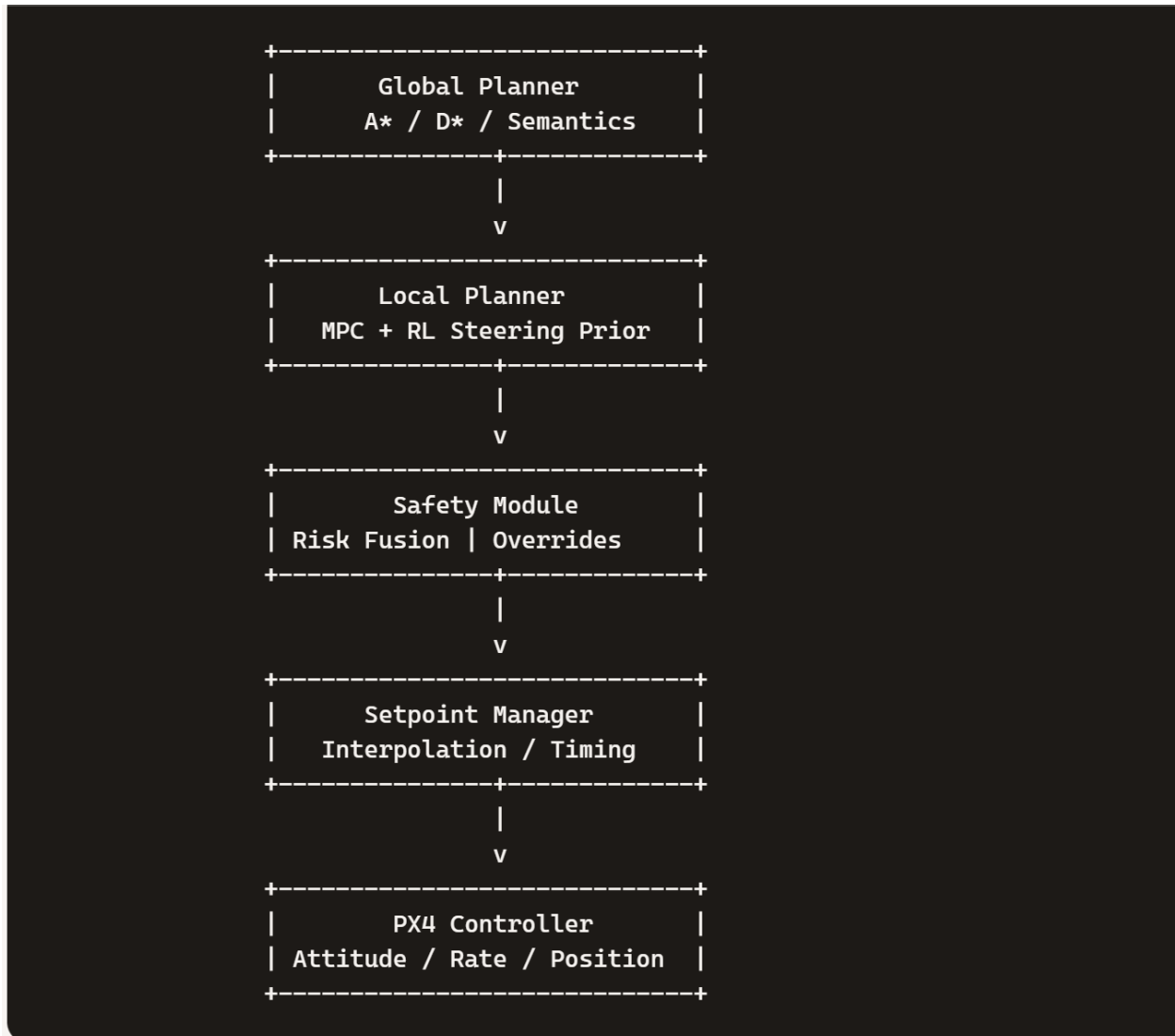
Fig. 10. Hierarchical interaction between planning, safety, and control modules in AUROUAV.
