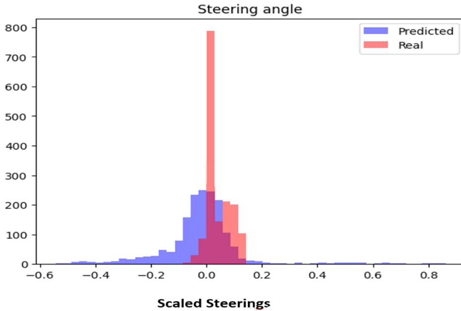
Fig. 17. Steering angle distribution for real (red) and predicted (blue) steering commands. The x-axis represents scaled steering observations, and the y-axis represents empirical likelihood.
